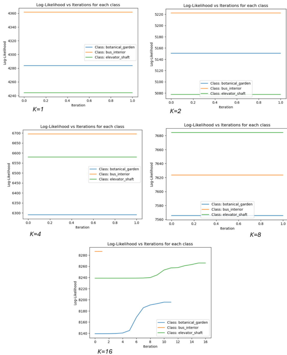
Figure 14 Log-Likelihood vs Iterations Plots
