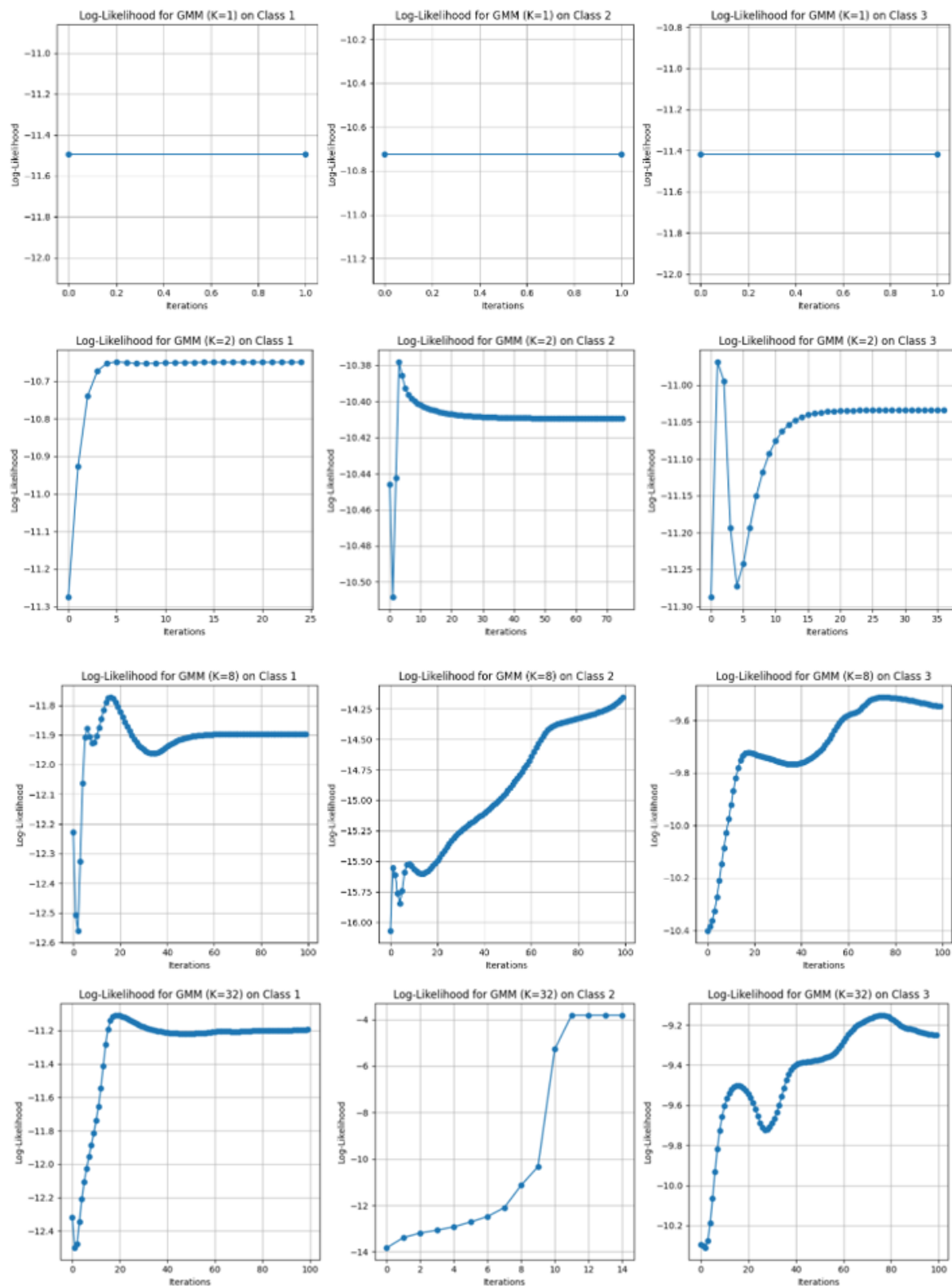
Figure 6 Log-Likelihood vs Iterations Plots for K = 1, 2, 8 and 32
