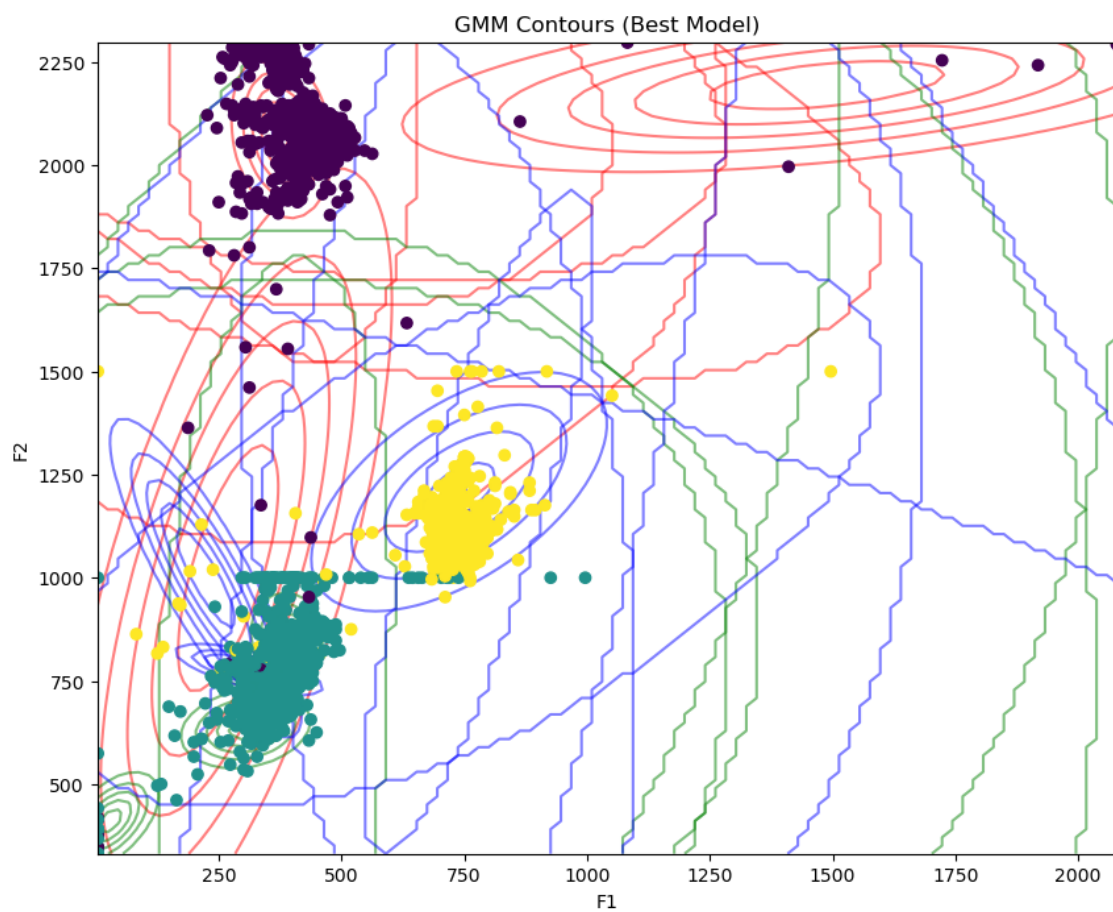
Figure 9 Constant Density Plot
