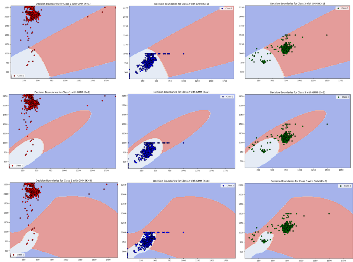
Figure 8 Decision Regions Plots
