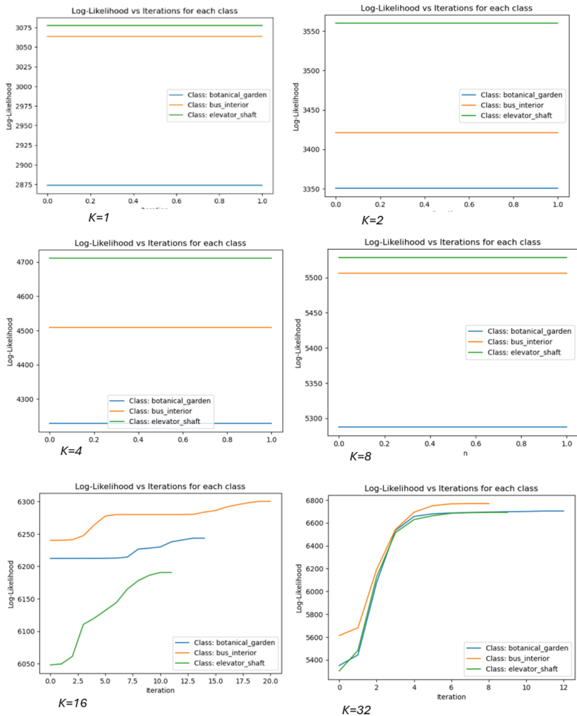
Figure 10 Log-Likelihood vs Iterations Plots
