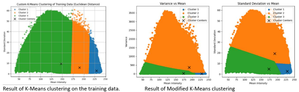
Figure 15 K Means vs Modified K-Means Clustering
