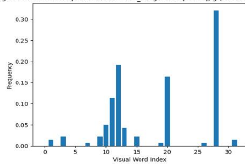
Bag of Visual Word Representation - sun_ategwvltlpxpobot.jpg (botanical_garden)
